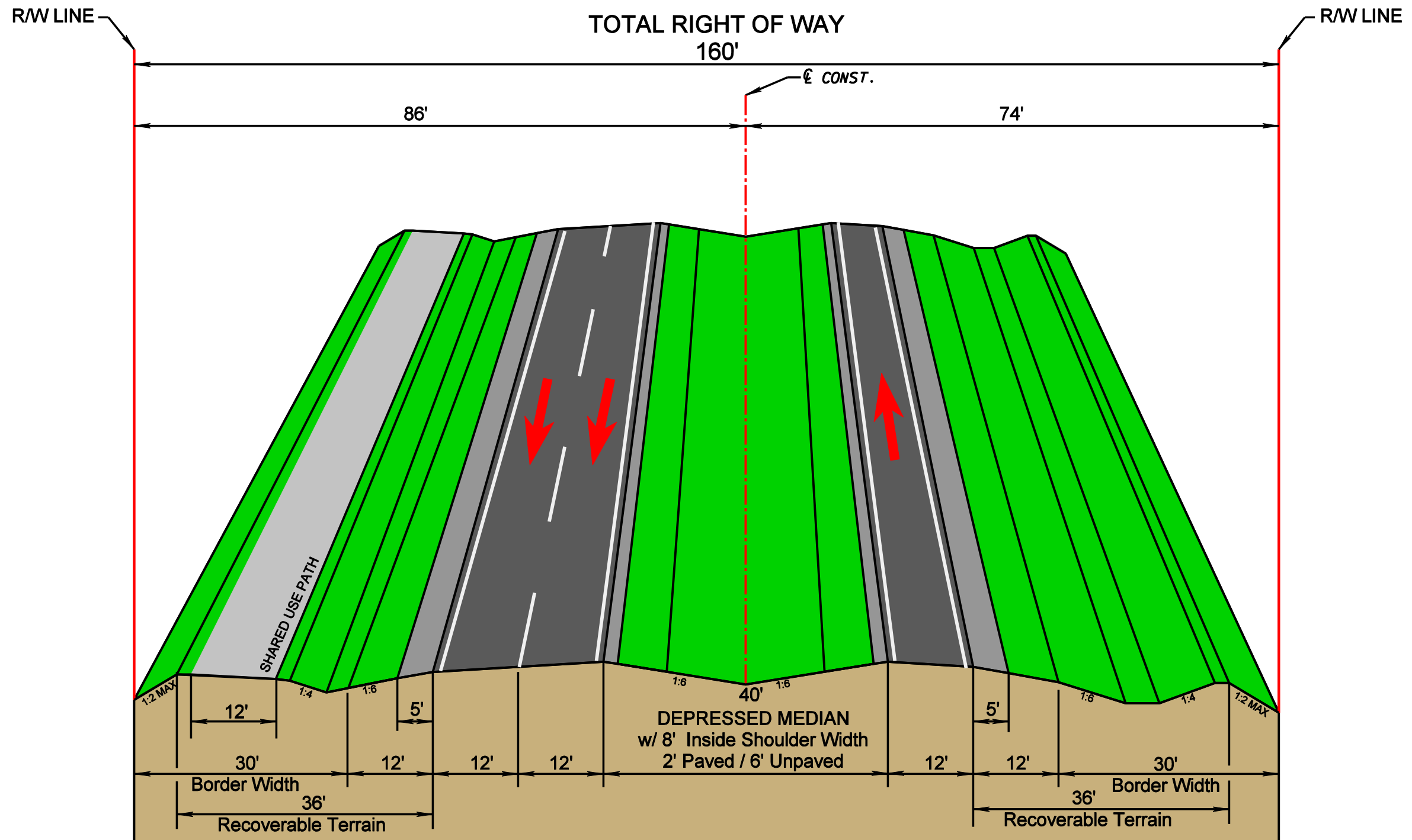
3- Lane Divided Roadway - Typical Section (Same As Alternative 1 With Passing Zones)
