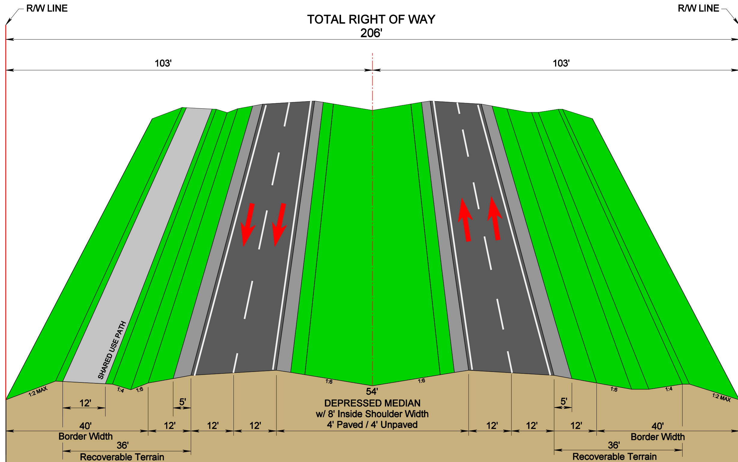
4- Lane Divided Roadway - Typical Section
